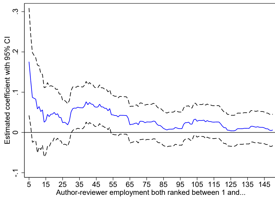
Figure A3: Author-reviewer employment rank match on positive evaluation by different rank cutoffs
