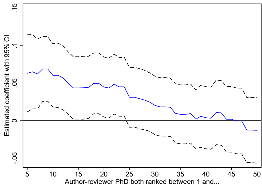
Figure A2: Author-reviewer PhD rank match on positive evaluation by different rank cutoffs
